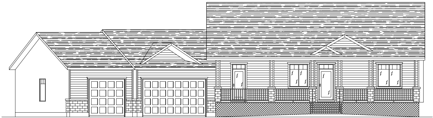
FRONT ELEVATION
